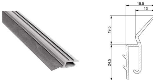
Cheder superior
